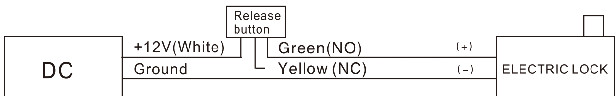
Fail-secure(chart1)
