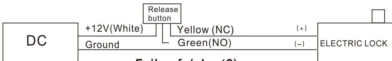
Fail-safe(chart2)
